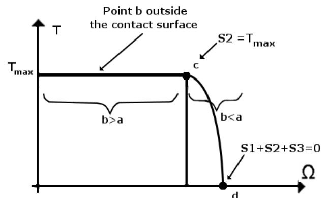
Fig. 6. Torque/speed curve
