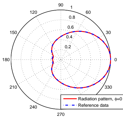
Fig. 5. Computed radiation pattern of DRA using near-to-far field transformation in the plane \phi = 0 .
