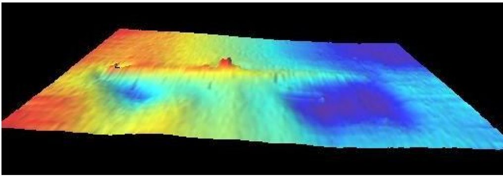
Fig. 7. Wreck on the bottom of the Gdansk Bay. Image from multibeam echosounder.
