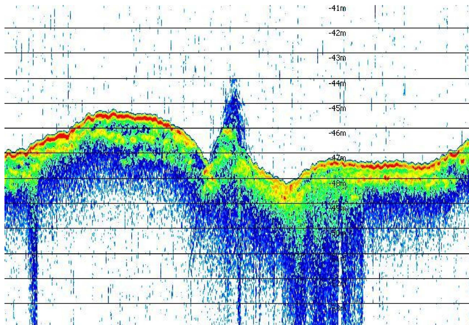
Fig. 8. Wreck on the bottom of the Gdansk Bay (the same as in Fig. 7). Image from parametric echosounder.
