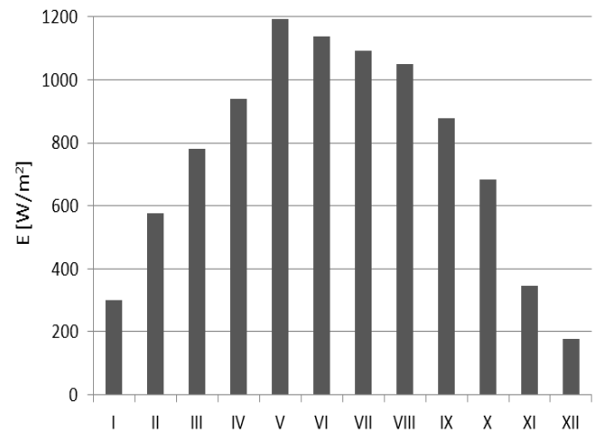
Figure 2: Maximum temporary solar irradiance during the year in Gdańsk (northern Poland) experimental data [6].
