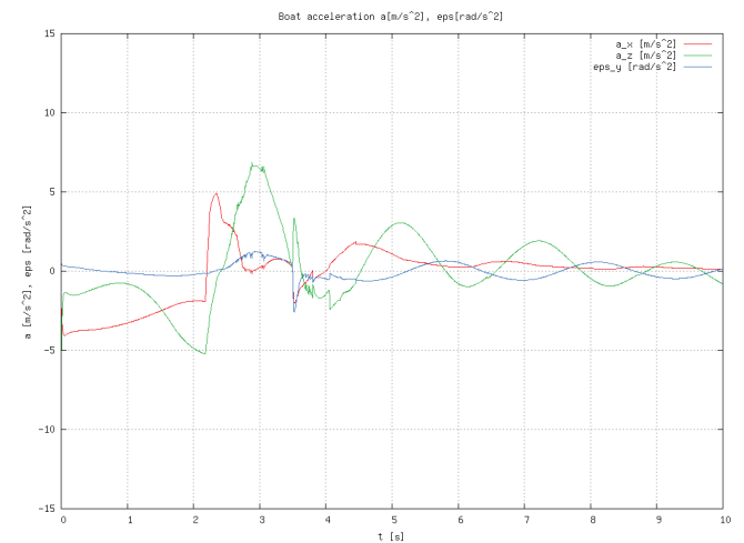
Fig. 5a. Module acceleration components: horizontal a_x , vertical a_z and angular \epsilon_z
