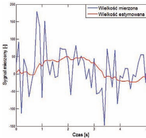
Rys. 14. Działanie filtra alfa-beta Fig. 14. Results of working alpha-beta filter
