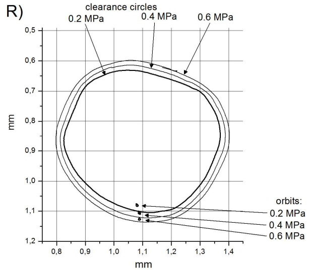
Fig. 12. Shaft orbits in measured clearance circles, bearing D for load 0.2 – 0.6 MPa, shaft revolution speed 11 rev/s
