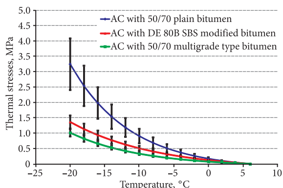
Fig. 5. Calculated thermal stresses induced in restrained asphalt concrete specimens by cooling with a rate of V_T = 10 \text{ °C/h}
