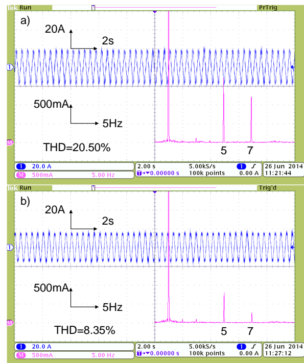
Fig.9. The harmonics and phase current waveform of a two-level VSI with compensation of dead-time effect using classic (a) and proposed compensation method (b). The frequency of output voltage vector: f=2.5\text{Hz} . Indicated: 5-th and 7-th harmonics of a phase current.
