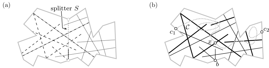
Fig. 21. (a) A subarrangement \tilde{\mathcal{A}} and its left (dashed) and right (dotted) segments with respect to a splitter S . (b) A splitter S , a (dotted gray) curve C and its (S, x) -separator (the black bold lines).
