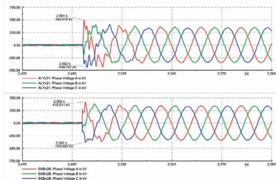
Fig. 6. Phase voltages at the ends of circuit II of EKB-ALY line
