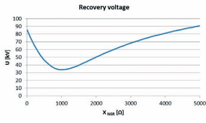
Fig. 9. Recovery voltage dependence on earthing reactance.
