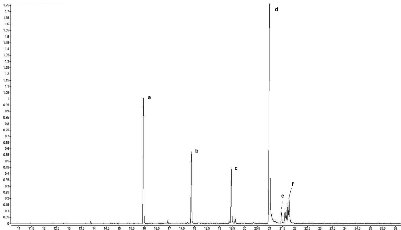
Fig. 9 Representative GC chromatogram of products of reaction; (a) – fatty acid C_{16} methyl ester; (b) – fatty acid C_{18} methyl ester; (c) – ketone 3 ; (d) – glycol 2 , (e) – epoxy oleic acid methyl ester; (f) – diepoxides and diglycols.
