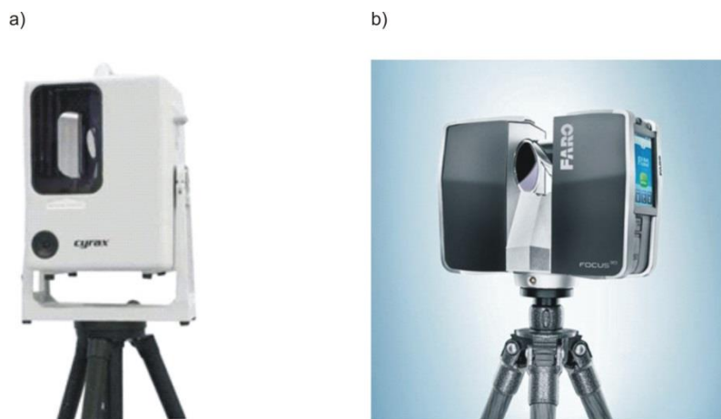
Rys. 3. Skanery laserowe: a) Cyrax 2500 [2], b) FARO Focus3D [1]
