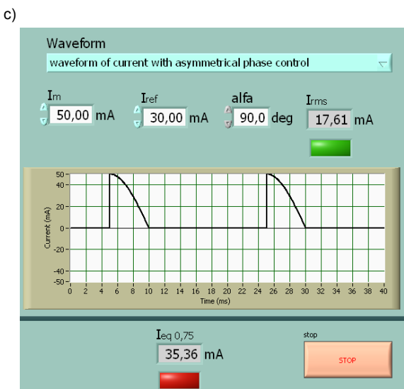
Fig.12. Front panel of the LabVIEW based computer system for analyse: a) half wave rectified current, b) alternating current with symmetrical phase control, c) current with asymmetrical phase control
