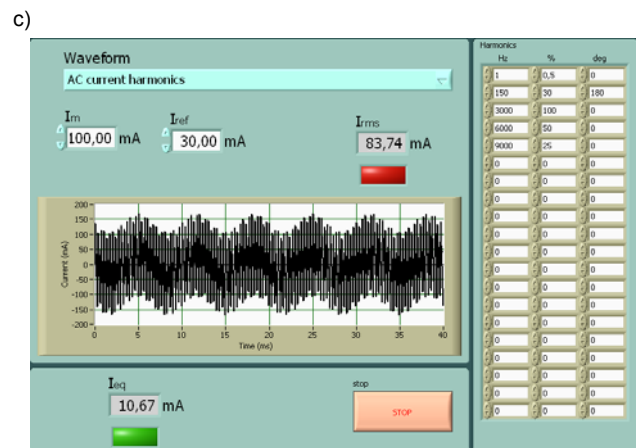
Fig.13. Front panel of the LabVIEW based computer system for analyse of earth current in variable speed drive circuit; PWM frequency 3 kHz: a) motor frequency 50 Hz, b) motor frequency 25 Hz, c) motor frequency 1 Hz
