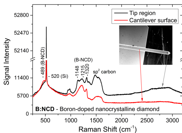
Fig. 5 Raman spectra of the silicon cantilevers coated with boron-doped diamond films—cantilever2
