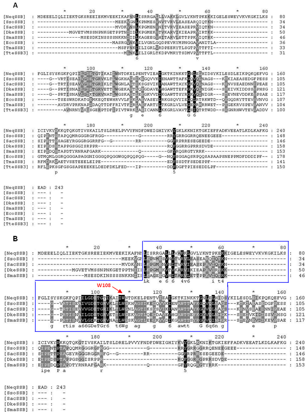
Fig 1. The multiple amino acid alignment. A The multiple amino acid alignment of nucleic acid binding protein from Nanoarchaeum equitans , bacterial and cruenarchaeal SSB proteins. B The multiple amino acid alignment of nucleic acid binding protein from Nanoarchaeum equitans and cruenarchaeal SSB proteins. The alignments were performed by dividing the amino acids into six similarity groups: group 1 V, L, I, M, group 2 W, F, Y, group 3 E, D, group 4 K, R, group 5 Q, D, and group 6 S, T. The capital letters represent single amino acid codes. White fonts on black boxes represent 100% similarity, white fonts on grey boxes denote <80% similarity, and black fonts on grey boxes show <60% similarity. Abbreviations: NeqSSB—nucleic acid binding protein from Nanoarchaeum equitans Kin-4M, SsoSSB Sulfolobus solfataricus strain P2, SacSSB Sulfolobus acidocaldarius DSM 639, SmaSSB Staphylothermus marinus F1, DkeSSB Desulfurococcus kamchatkensis 1221n, EcoSSB Escherichia coli K12, TmaSSB Thermotoga maritima strain MSB8, and TteSSB3 Thermoanaerobacter tengcongensis MB4. The W108 residue, important in base-stacking interactions is indicated in the panel B. The blue box indicates OB-fold region.
