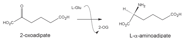
Figure 1. Reaction catalyzed by \alpha -amino adipate aminotransferase.
