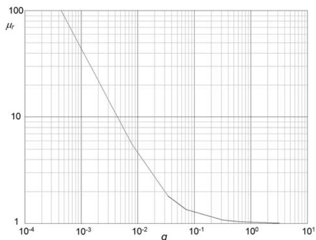
Fig. 4. Calculated dependence between equivalent, relative permeability of the magnetically contaminated layer of an amagnetic cylinder and relative density of magnetic contamination (for the initial value \mu_r = 100 and g = 5 \cdot 10^{-4} ).
