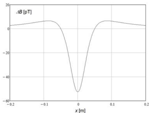
Fig. 3. Disturbance in the distribution of the magnetic flux density caused by a ferromagnetic layer with the thickness R_2 - R_1 = 10 nm on the amagnetic cylinder with the radius R_1 (for H_o = 39.788 A/m, \mu_r = 100 )
