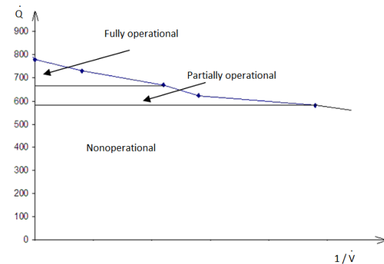
Fig. 6. Three-level evaluation of the diesel oil cooler technical condition
