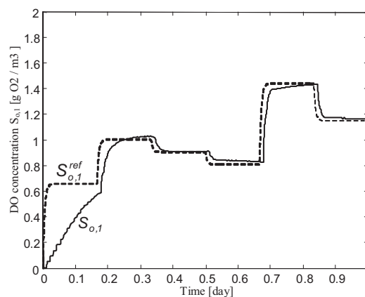
Fig. 13. DO concentration in aeration tank 1 – control system 2
