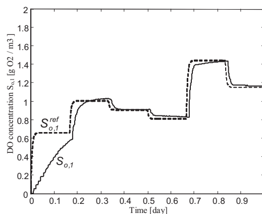
Fig. 15. DO concentration in aeration tank 2 – control system 2
