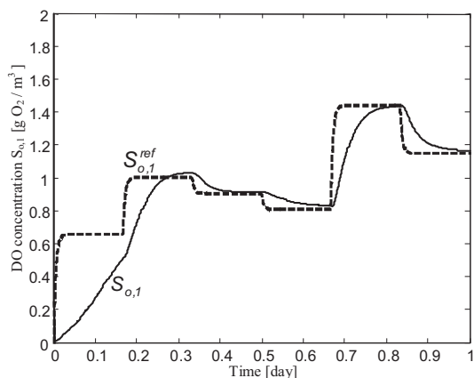
Fig. 12. DO concentration in aeration tank 1 – control system 1
