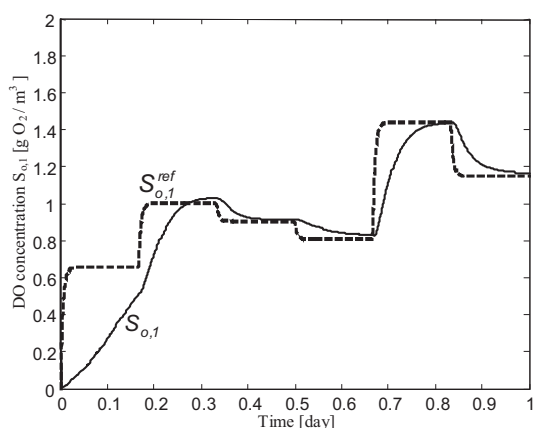
Fig. 14. DO concentration in aeration tank 2 – control system 1
