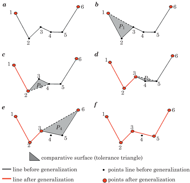
Fig. 1. Stages in line generalization based on comparative surface
