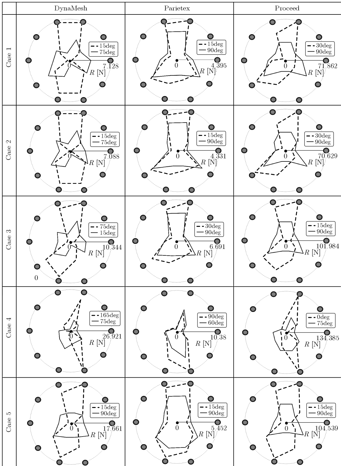
Fig. 5. Reactions F obtained in each support for all investigated orientations of the implant, the solid line is for the best orientation, the dashed line is for the worst orientation of the mesh
