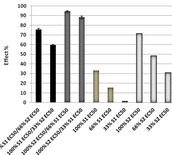
Fig. 7 Results obtained for the mixture of gemfibrozil (S1) and diclofenac (sodium salt) (S2)
