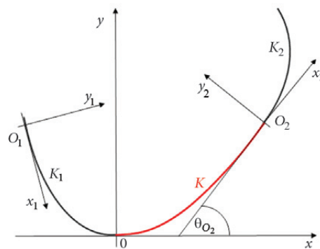
Fig. 1. Schema of the geometrical route layout
