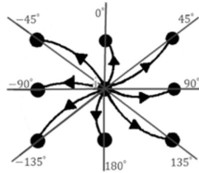
Figure 6. The angles \beta \in B were assigned to the outgoing edges of the vertex i
