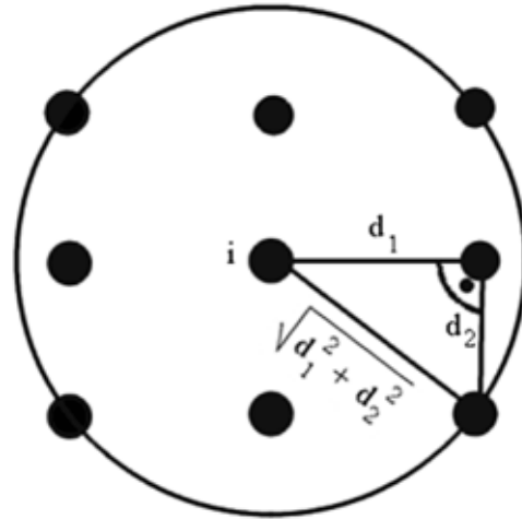
Figure 2. Vertex i and its neighbors
