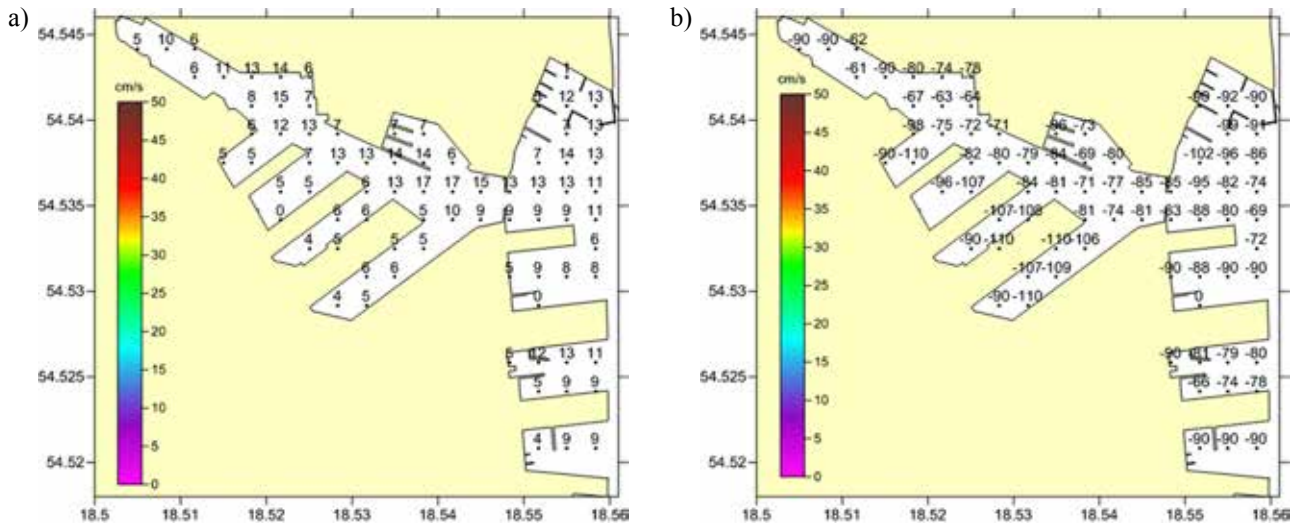
Figure 7. Data on the surface currents in the waters of Gdynia harbor as designated in the hydrodynamic M3D model: a) current speeds, b) current directions
