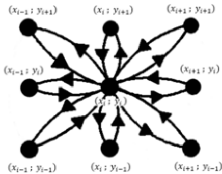
Figure 5. Vertex i with node (x_i, y_i) and its neighbors, with their corresponding nodes, in the discretization grid
