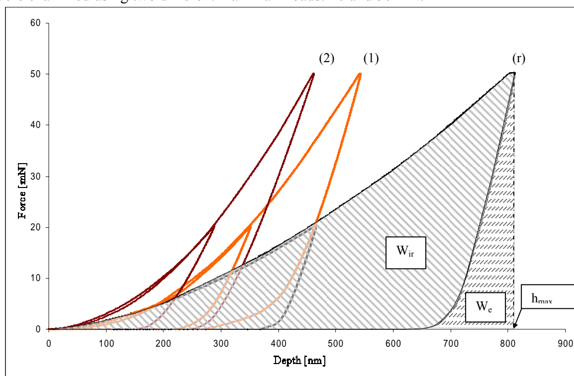
Fig. 5. Force – indentation depth curves measured on the surface of nitride layers after processes: no. 1 (1), no. 2 (2). Results were compared with the reference material (r)
