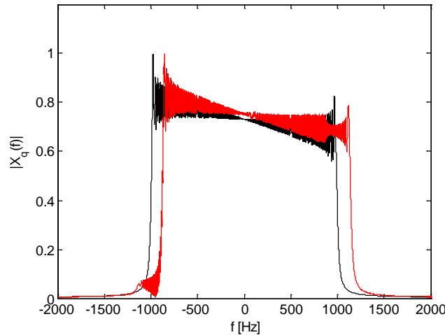
Fig. 1. Spectrum of the sounding signal (black) and echo signal (red) ( f_o = 10 kHz, B = 2 kHz, T = 2 s, f_s = f_o/2 , v = 10 m/s, c = 1500 m/s).
