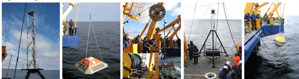
Fig. 1. Photographs of the equipment used during RUN A40. From left to right: receive tower with seven hydrophones, ADCP turtle, towed CTD chain with 85 sensors, transmit tower, and waverider buoy.
