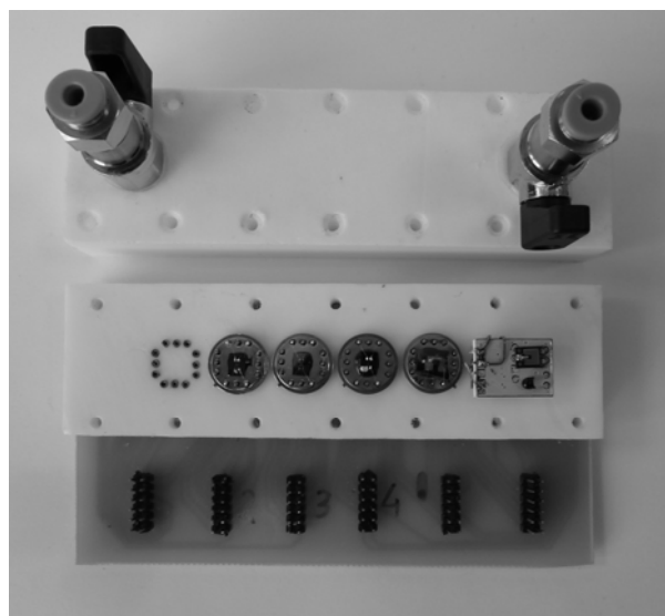
Fig.4. Picture of the prepared gas chamber made of Teflon: a substrate with a set of four gas sensors and integrated control of environmental parameters (center), connector to the sensors' terminals (bottom) and a second part of the chamber with the valves (top); the chamber is screwed using a silicone gasket to avoid eventual leakage
