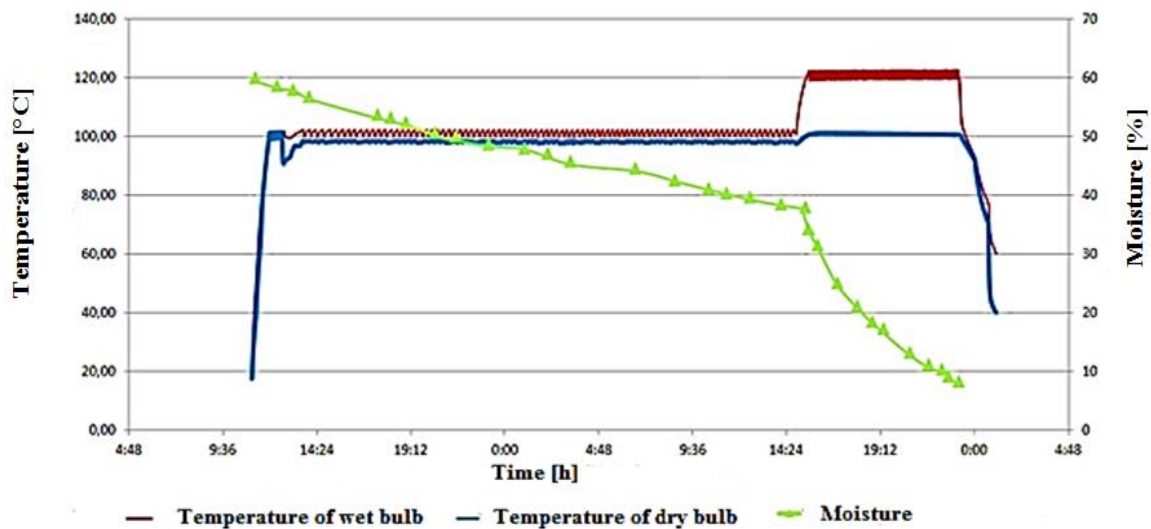
Fig. 6. Variable changes during high temperature drying
