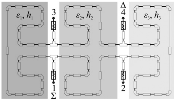
Fig. 3 Design case 1: Layout of the compact RRC composed of folded TLs
