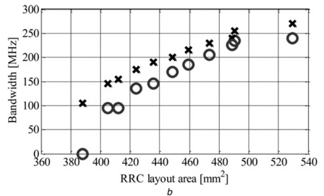
Fig. 4 Design case 1: Pareto set representations found by means of
