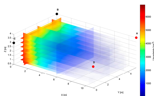
Figure 7. Volumetric slice plot of uncertainty-precision distribution for location sensors AD .
