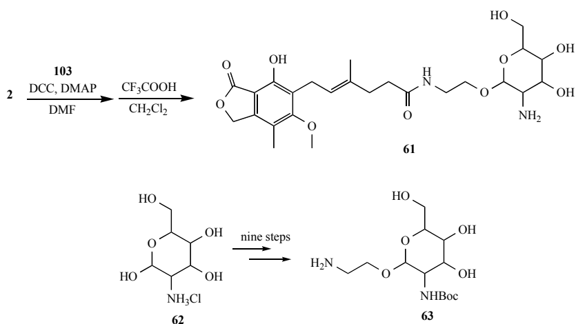
Scheme (5). Synthesis of a conjugate of mycophenolic acid with glucosamine 61 [40].
