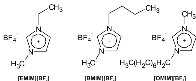
Fig. 1. Structure of 1-ethyl-3-methylimidazolium tetrafluoroborate [EMIM][BF 4 ], 1-butyl-3-methylimidazolium tetrafluoroborate [BMIM][BF 4 ] and 3-methyl-1-octylimidazolium tetrafluoroborate [OMIM][BF 4 ] ionic liquids used for NTs formation.
