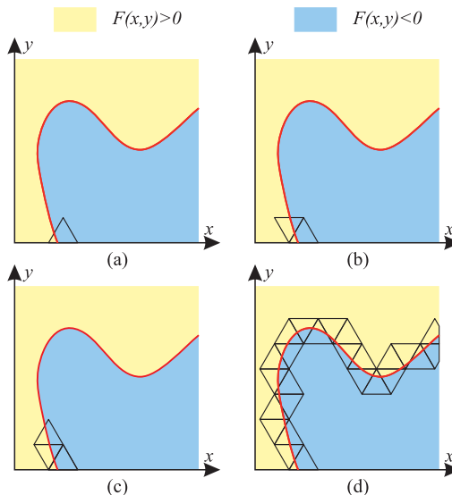
Fig. 1. Example of a root tracing process in real 2-D case [2], [3]. (a)–(c) First three steps. (d) Final result.
