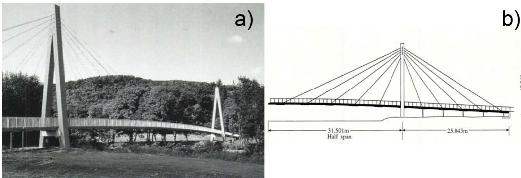
Fig. 2. Footbridge in Aberfeldy, UK: a) view, b) half of the structure elevation; (Source: Harvey 1993)
