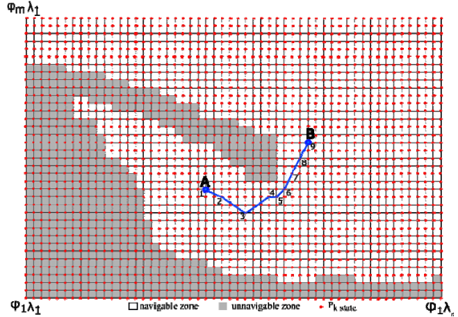
Figure 2. Described chart with constant granularity of area with example of route from start point A to finish point B with 32 possible movements of a sailing vessel from each point P_k , illustrated are 9 points P_k , where in point designed by 7, 8, 9 is course
