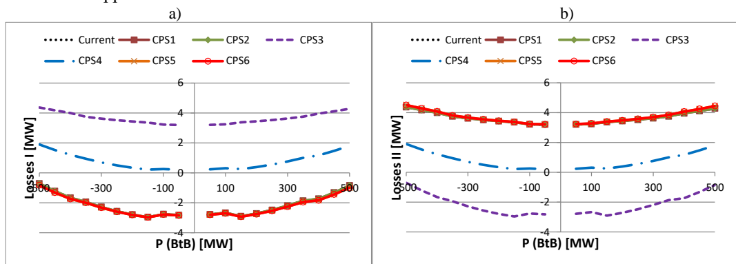
Fig. 11. Active power losses for different phase sequence, a) Circuit I, b) Circuit II.
