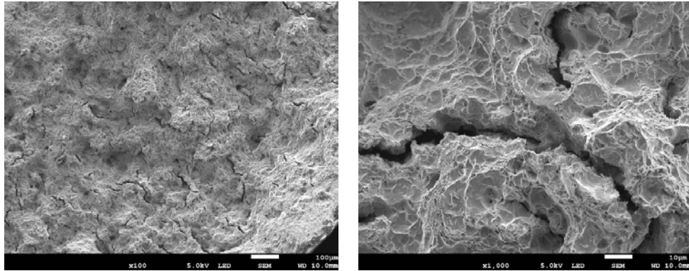
Fig. 7. The fracture faces of the specimens oxidized at 350°C and: a, b) simultaneously hydrogen charged at 80 mA/cm 2 and tensed; c, d) hydrogen charged at 80 mA/cm 2 for 72 h, heated at 400°C for 4 h and then tensed
