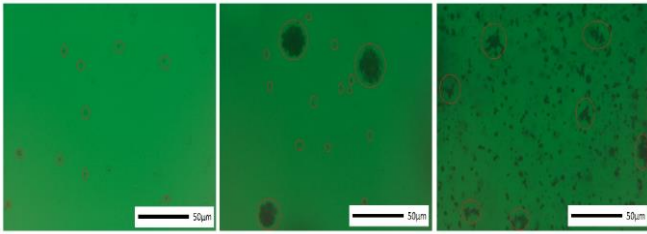
Fig. 6. Comparison of the distribution of nanocopper agglomeration using different bases, i.e.: alcohol, contact lenses liquid, olive in double dipping for 5 seconds [500x]
