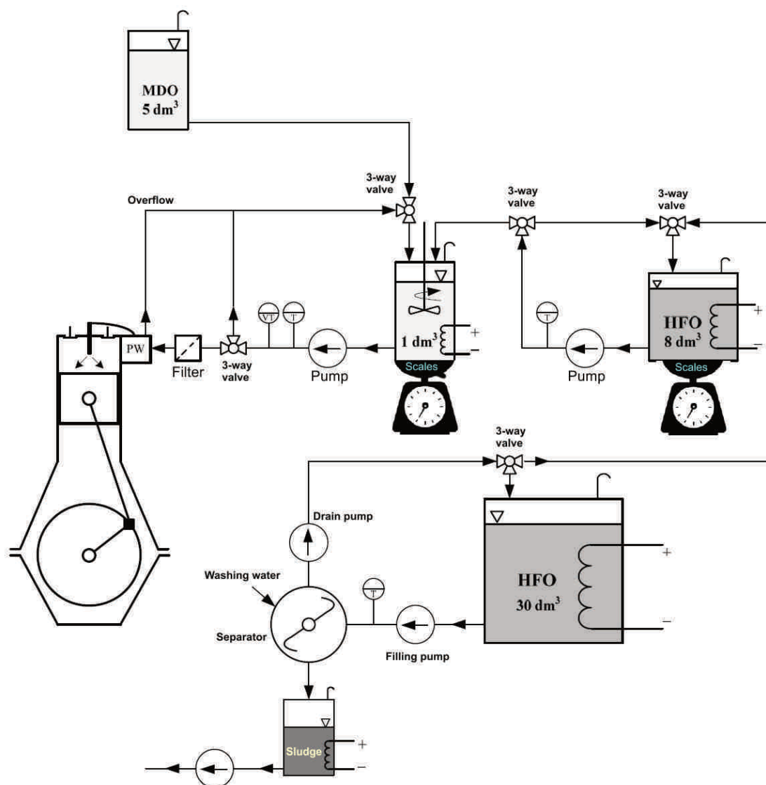
Fig. 2. Conceptual scheme of installation of supplying the laboratory engine Farymann Diesel type D10 with fuel oil: MDO – Marine Diesel Oil; HFO – Heavy Fuel Oil; PW – injection pump, VT – viscometer, T – thermometer
