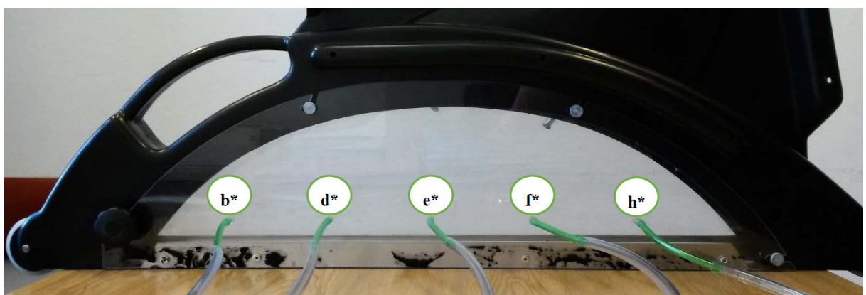
Figure 2. Location of measurement points on a narrow cover
