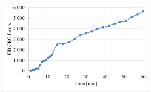
Fig. 7. Multiplex FIB CRC Errors.
