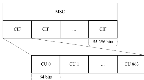
Fig. 2. An inner structure of MSC.
