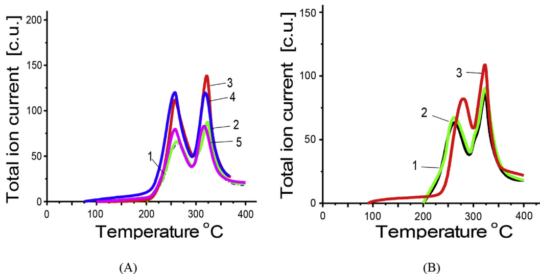
Fig. 5. Curves of changes in the total ion current as a function of temperature during thermodestruction of Tecoflex® before (1-EG control; A) and after incubation in NB medium (2-EGNB; A) in microorganism cultures: Bacillus subtilis (3-EGBs; A), Ps.denitrificans (5-EGPd; A) and Ps.fluorescens (4-EGPf; A) and before (1-EGcontrol; B), and after incubation in medium SB (2-EGSB; B), in culture Yar. lipolytica (3-EGYI; B) five months.
