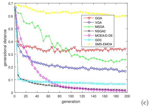
Fig. 2. Original indicators for the seven unattended EMOO algorithms in their averaged simulation runs [23]: (a) Hyper Volume; (b) Spacing, (c) Generational Distance.
