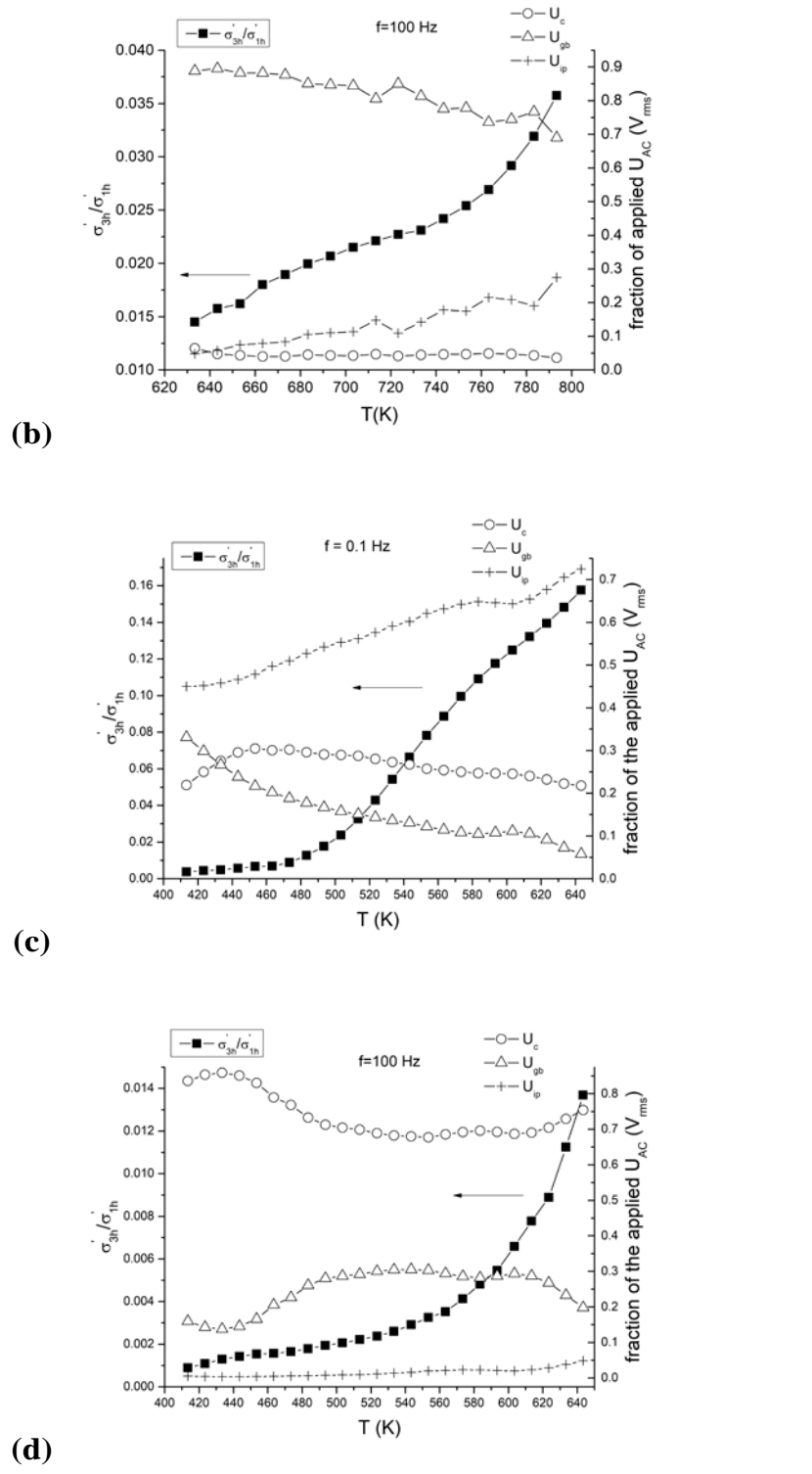
Figure 3 The temperature dependence of the fraction of applied A.C. voltage that dropped over three regions ( U_c , U_{gb} , U_{ip} ) and the ratio of the third harmonic to the base conductivity for 50BiV-50SrBAIO nanocomposite ((a) 0.1 Hz and (b) 100 Hz) and BiV ceramic ((c) 0.1 Hz and (d) 100 Hz). The U_c is the A.C. voltage fraction calculated for Bi_2VO_{5.5} nanocrystallites (in
