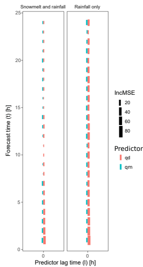
Figure 9. Importance of the discharge-based predictors used in the Random Forests models (Equations (1) and (2)) for the snowmelt and rainfall (left panel) and rainfall only (right panel) model variants. The vertical axis presents different forecast time t \in \langle 1; 24 \rangle h; the horizontal axis presents the predictor lag time l \in \langle -24; t \rangle h, which is always equal to 0 for this group of predictors. The area of the rectangles is proportional to the increase of the mean squared error (IncMSE) of Random Forests model after perturbing a predictor in reference to an original predictor, i.e., the higher the increase of the mean squared error the higher the predictor importance for a model. Red rectangles present the discharge difference ( qd ) predictor and the blue rectangles the mean discharge ( qm ) predictor (see Section 2.1).
