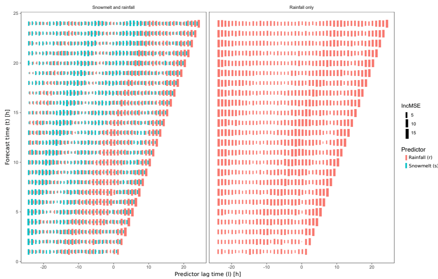
Figure 8. Importance of the forecasted meteorological predictors used in the Random Forests models (Equations (1) and (2)) for snowmelt and rainfall (left panel) and rainfall only (right panel) model variants. The vertical axis presents different forecast time t \in \langle 1; 24 \rangle h; the horizontal axis presents the predictor lag time l \in \langle -24; t \rangle h. The area of the rectangles is proportional to increase of the mean squared error (IncMSE) of Random Forests model after perturbing a predictor in reference to an original predictor, i.e., the higher the increase of the mean squared error, the higher the predictor importance for a model. Red rectangles present rainfall predictors ( r_l ) and the blue rectangles present the snowmelt predictors ( s_l ).
