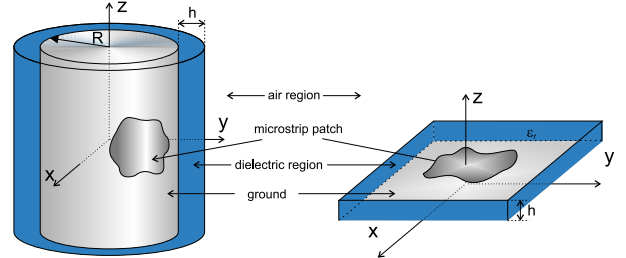
Fig. 1. The geometry of the investigated structures.
