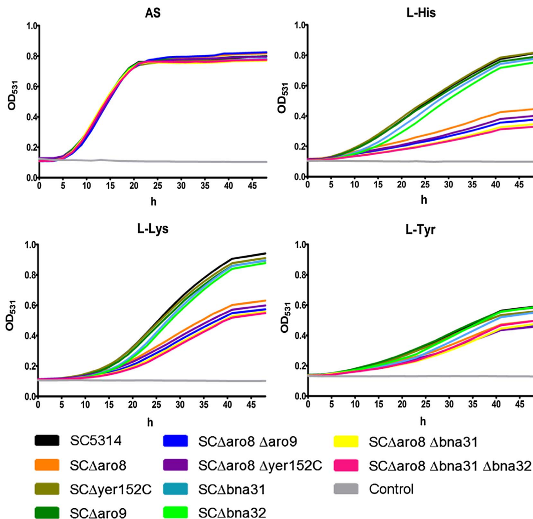
Fig. 3. Growth kinetics of C. albicans wild-type and deletion mutants in the YNB media containing either L-Lys, L-His, or L-Tyr as the sole nitrogen source (10 mM) or ammonium sulphate (AS). Cell density was measured at time intervals spectrophotometrically ( \lambda = 531 nm). Optical density of liquid medium (YNB) serves as a negative control.
