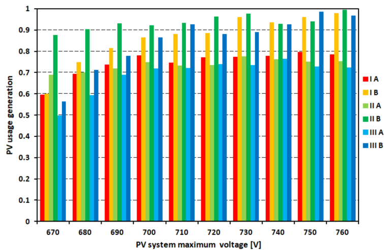
Figure 13. Utilization of the energy generation potential in the maximum generated voltage function of the PV system.
